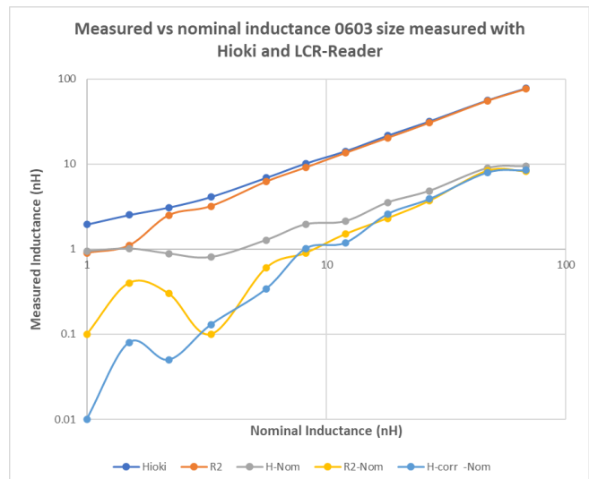
Figure 7. Inductance of 0603 components measured using LCR-Reader R2 with and without short calibration using Short Calibration Board. Compared to measurement results using Hioki IM3536 with and without test fixture offset subtraction.
